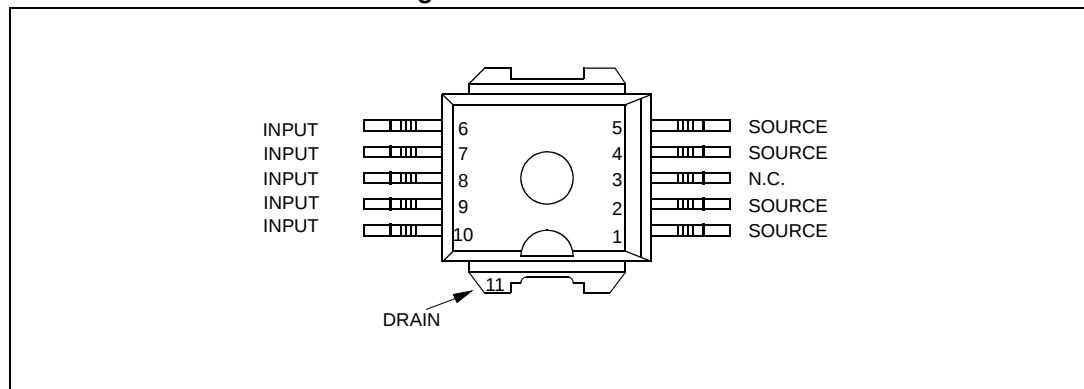
Figure 2. Pin connection
