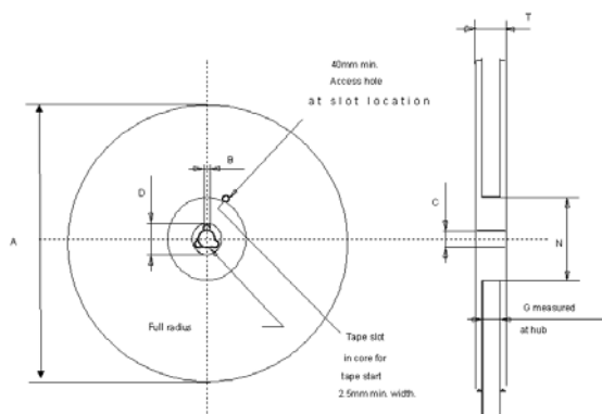
Figure 40. Tape and reel shipment (suffix “13TR”)
