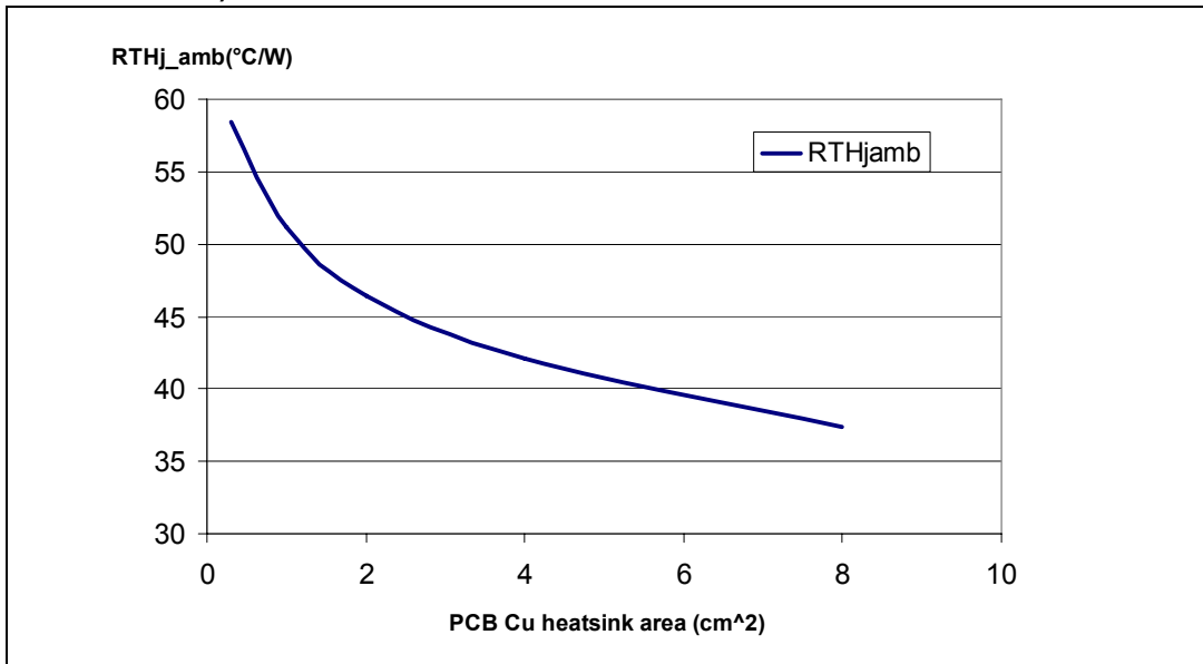
Figure 33. R_{thj-amb} vs PCB copper area in open box free air condition (one channel ON)
