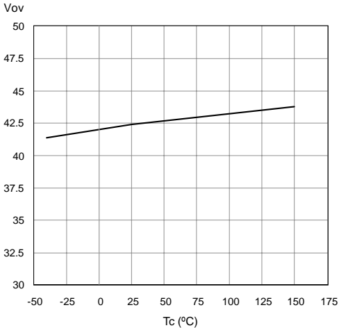
Figure 25. Overvoltage Shutdown
