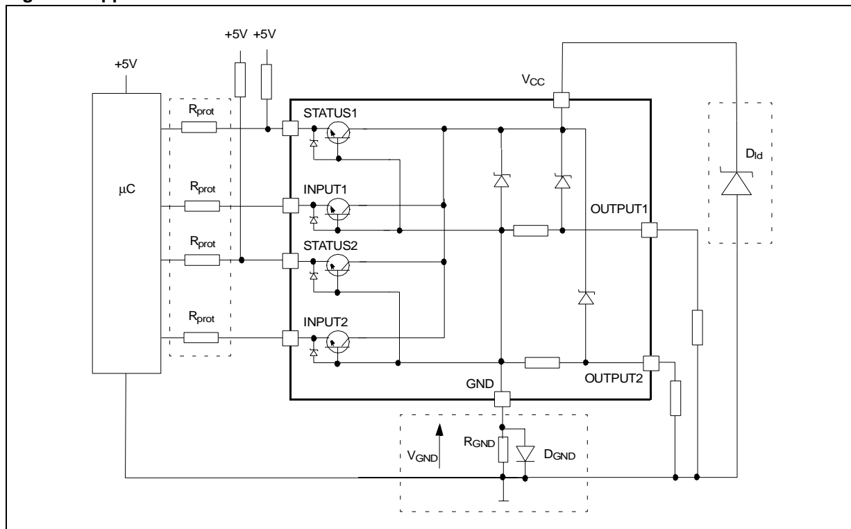
Figure 8. Application Schematic
