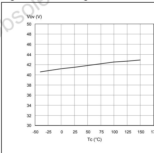
Figure 11. Overvoltage shutdown
