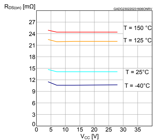
Figure 23. On-state resistance vs. V_{CC}
