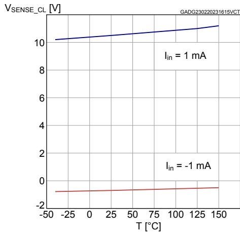
Figure 30. V_{sense\ clamp} vs. T_{case}
