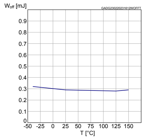
Figure 27. W off vs. T case
