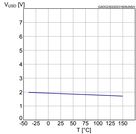
Figure 21. Undervoltage shutdown
