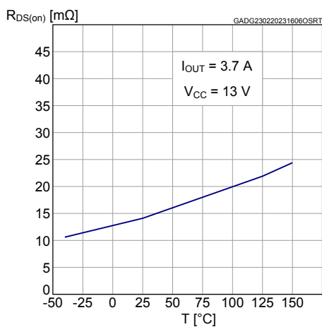
Figure 22. On-state resistance vs. T_{case}
