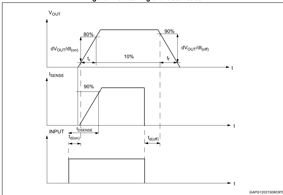
Figure 4. Switching characteristics
