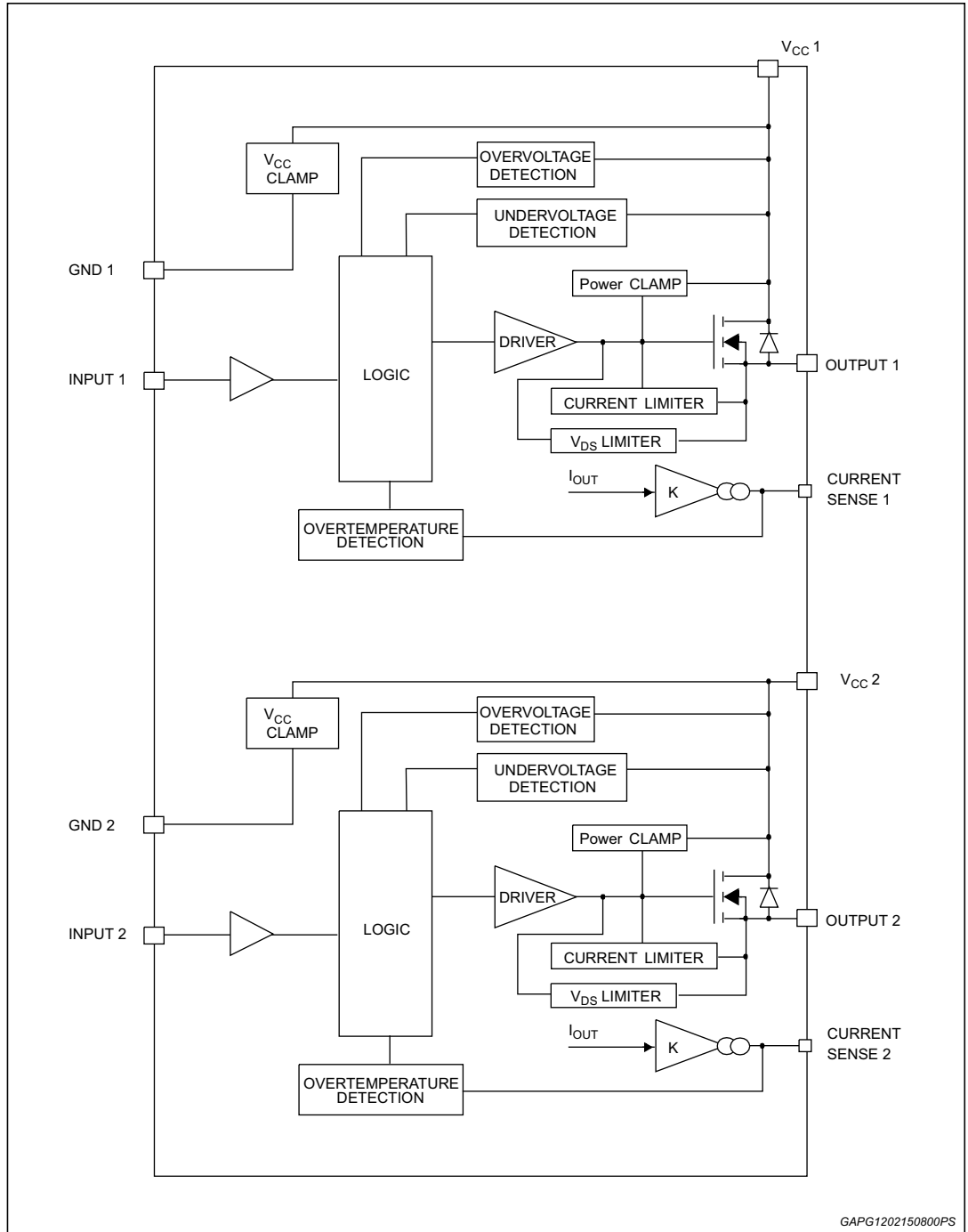
Figure 1. Block diagram
