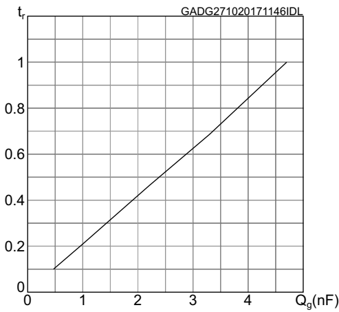
Figure 14. Gate driver low side rise time normalized vs C_g = 4.7\text{nF}
