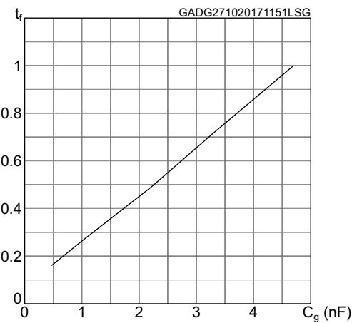
Figure 15. Gate driver low side fall time normalized vs C_g = 4.7\text{nF}
