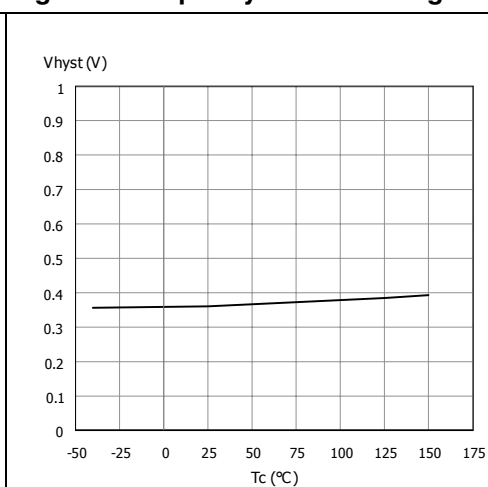
Figure 15. Input hysteresis voltage
