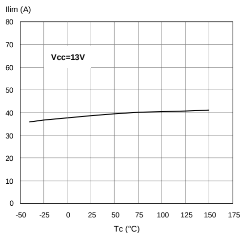
Figure 16. I_{LIM} Vs T_{case}
