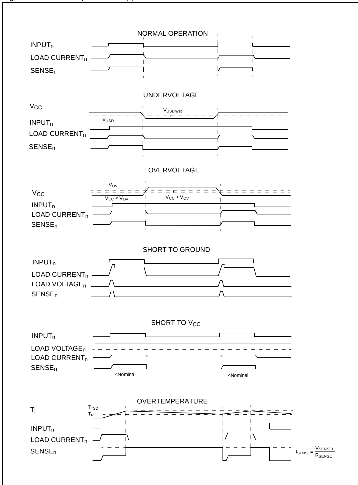
Figure 7. Waveforms (Per each chip)
