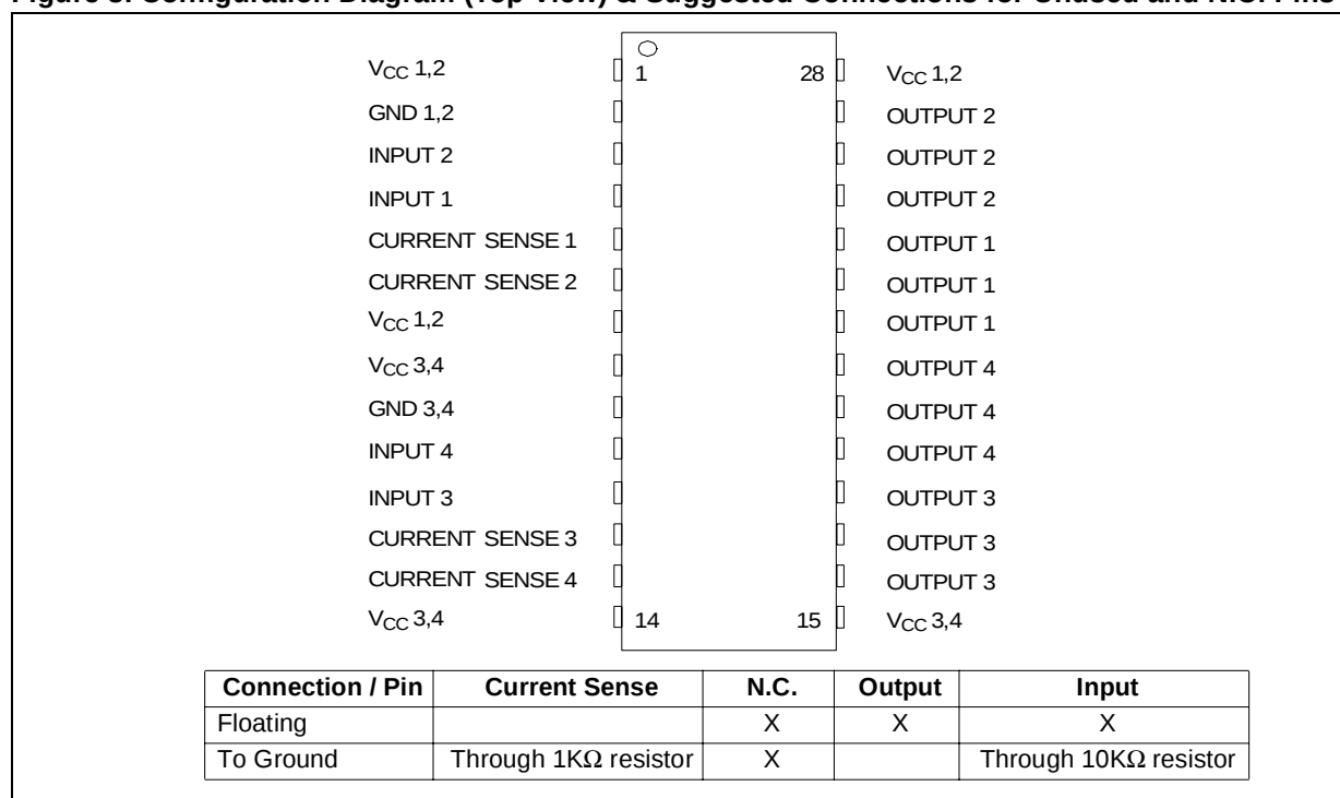
Figure 3. Configuration Diagram (Top View) &amp; Suggested Connections for Unused and N.C. Pins
