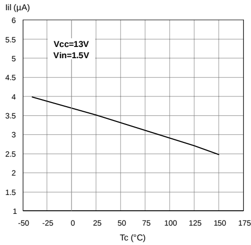
Figure 10. Low Level Input Current
