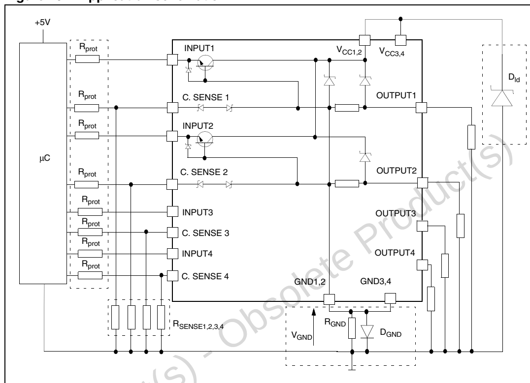
Figure 19. Application schematic
