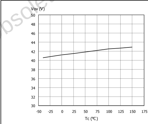
Figure 11. Overvoltage shutdown
