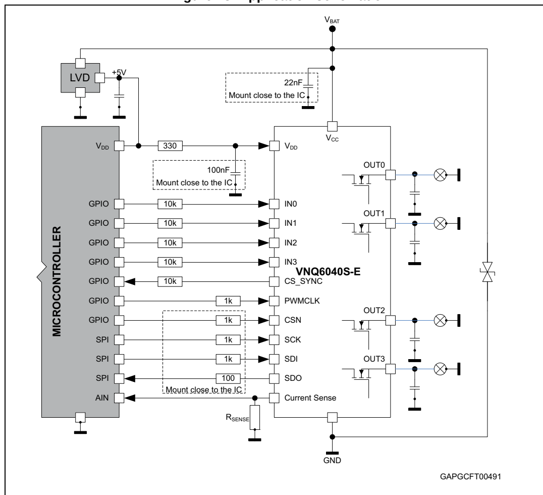
Figure 23. Application schematic
