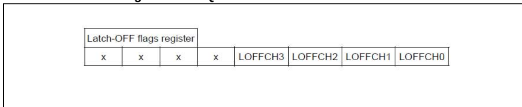
Figure 23. VNQ7003SY CHLOFFSR
