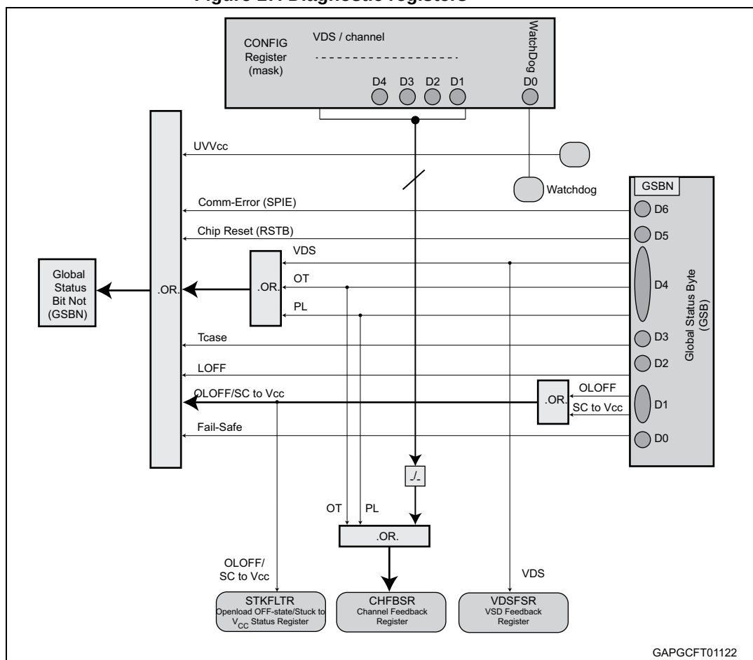
Figure 17. Diagnostic registers
