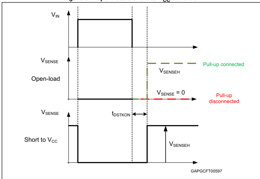
Figure 37. Open-load / short to V_{CC} condition
