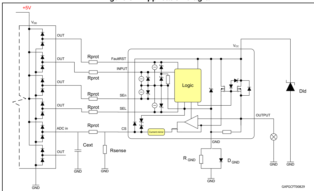
Figure 32. Application diagram
