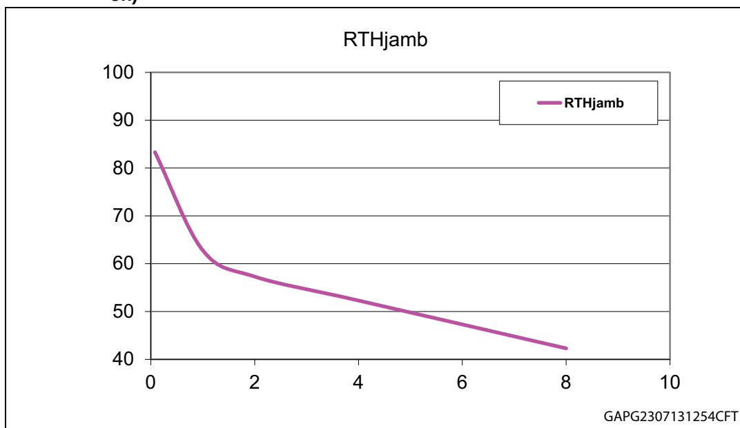
Figure 41. R_{thj-amb} vs PCB copper area in open box free air condition (one channel on)
