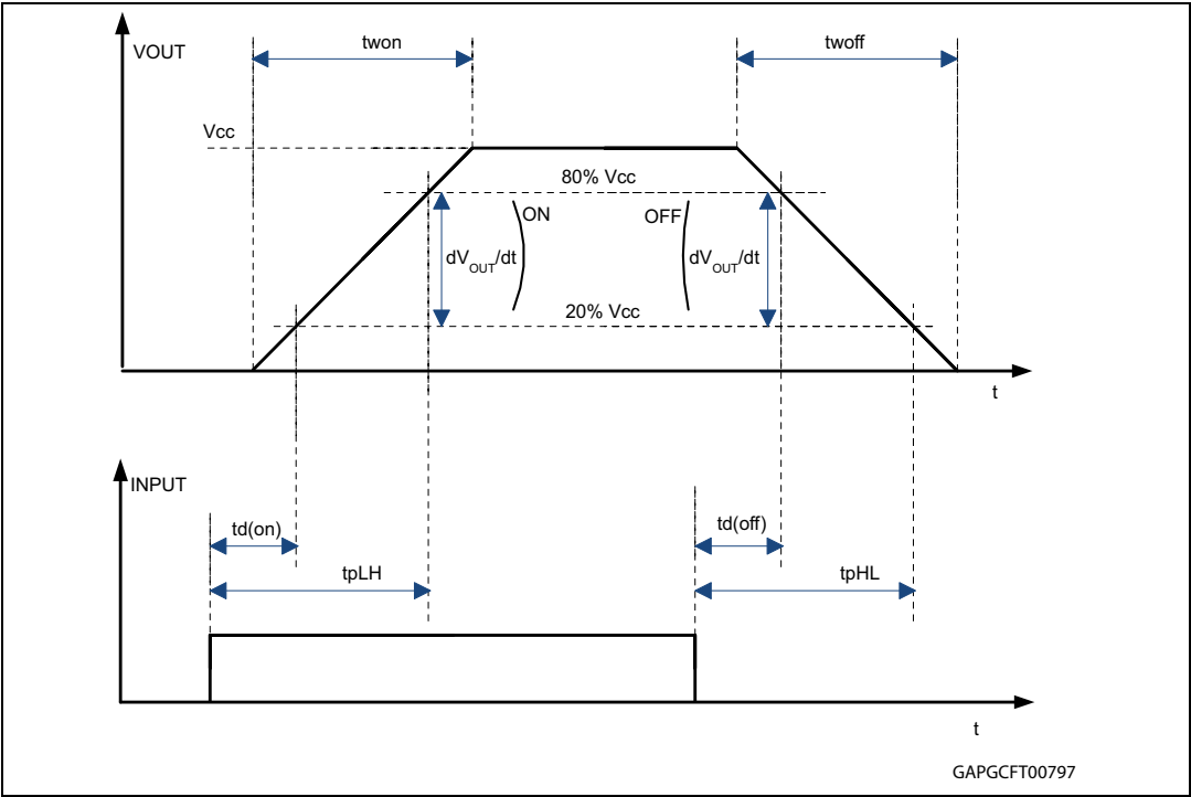
Figure 4. Switching times and Pulse skew
