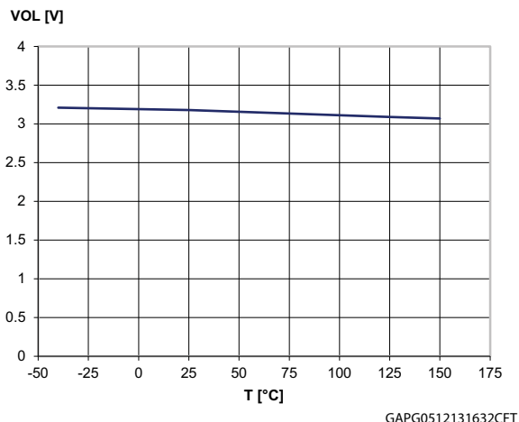
Figure 29. OFF-state open-load voltage detection threshold
