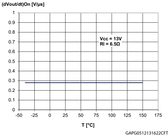
Figure 26. W on vs T case
