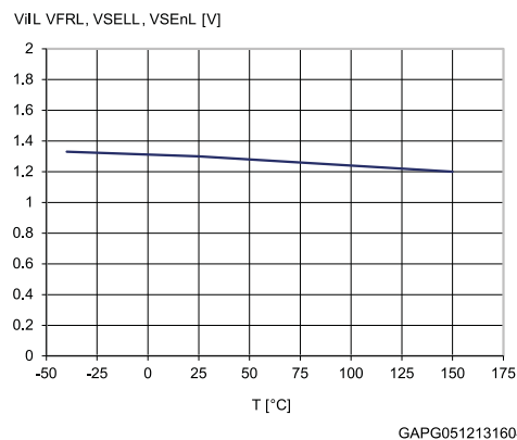
Figure 16: Logic Input low level voltage
