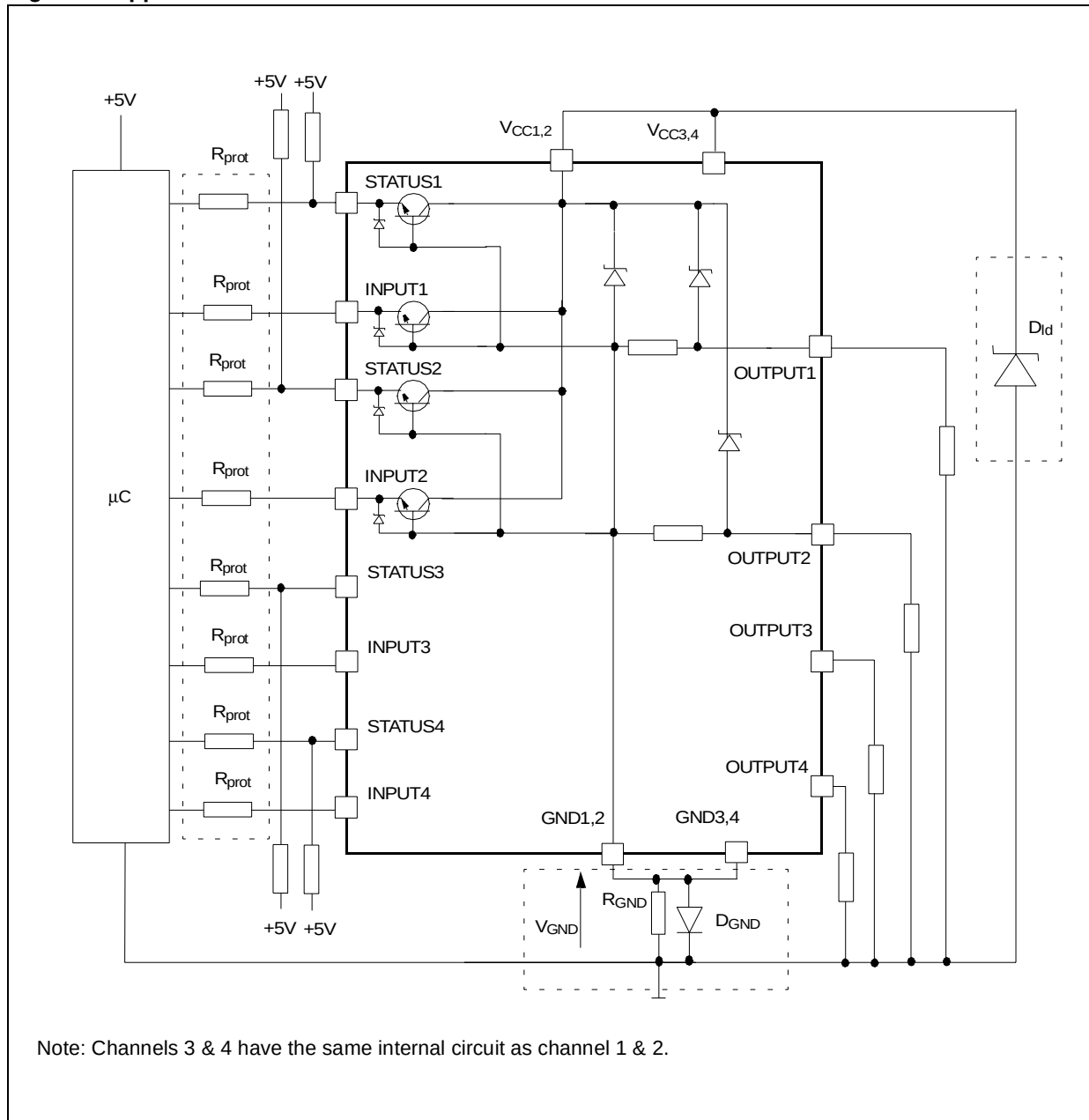
Figure 8. Application Schematic
