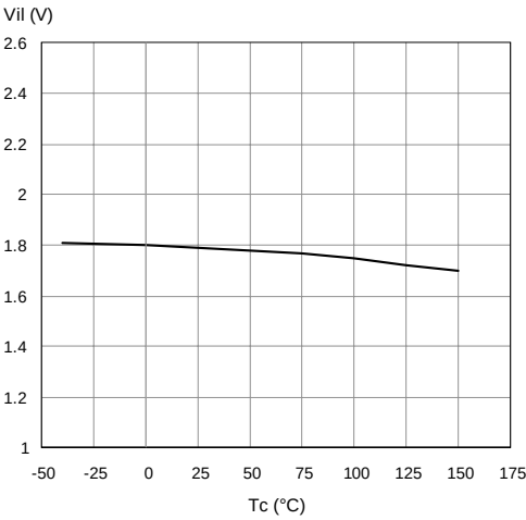
Figure 25. Input Low Level
