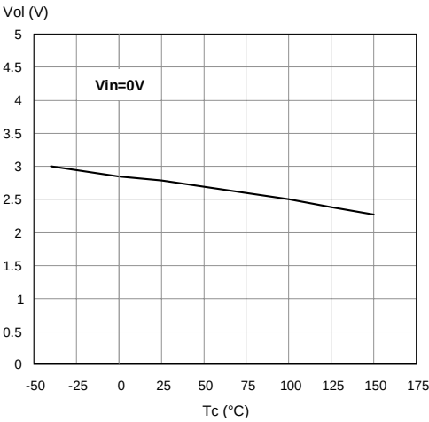
Figure 26. Openload Off State Detection Threshold
