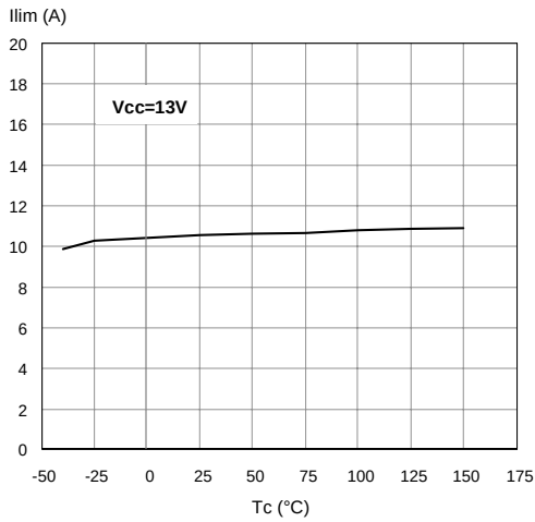
Figure 26. I_{LIM} Vs T_{case}
