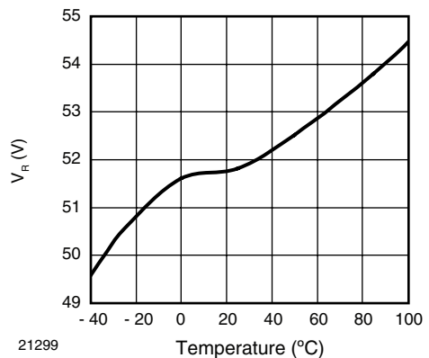
Fig. 5 - Diode Reverse Voltage vs. Temperature
