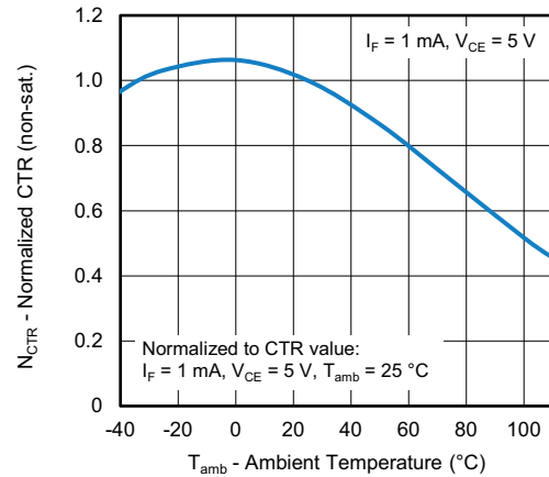
Fig. 10 - Normalized CTR (non-sat.) vs. Ambient Temperature
