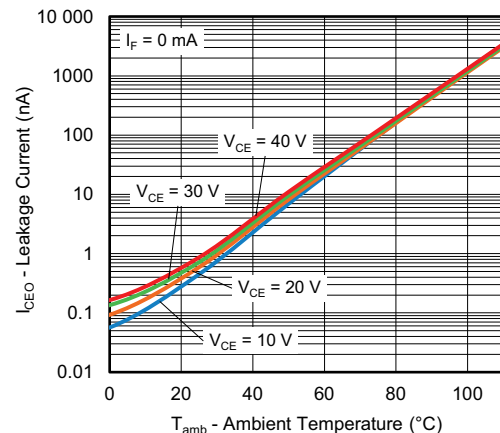
Fig. 12 - Leakage Current vs. Ambient Temperature
