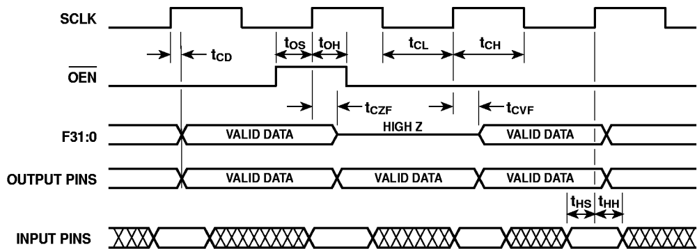
Fig. 21 Operating timings
