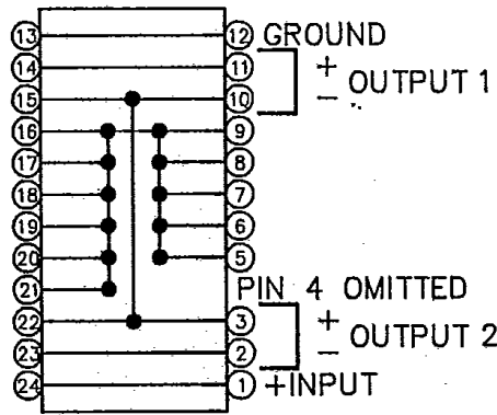
TOP VIEW VC
