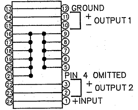
TOP VIEW VD
