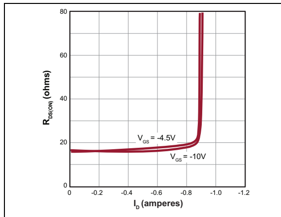
FIGURE 2-4: On-resistance vs. Drain Current.
