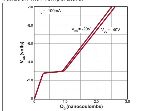
FIGURE 2-6: Gate Drive Dynamic Characteristics.
