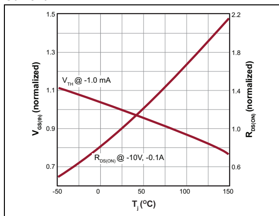
FIGURE 2-5: V_{GS(th)} and R_{DS(ON)} Variation with Temperature.
