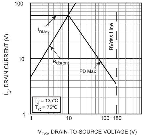
FIGURE 4, Forward Safe Operating Area
