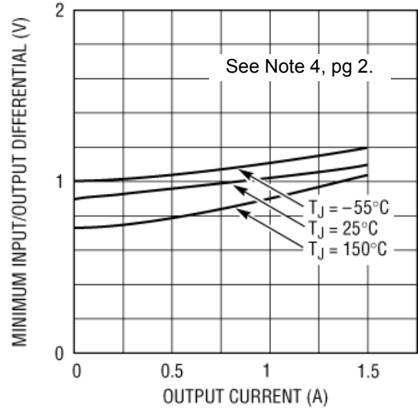
FIGURE 4 – RH1086 TYPICAL DROPOUT VOLTAGE CURVE
