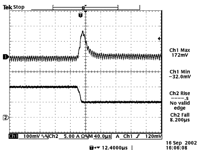
Vout=2.0V 100% to 50% load transients at 12V input and Ta=25° C
