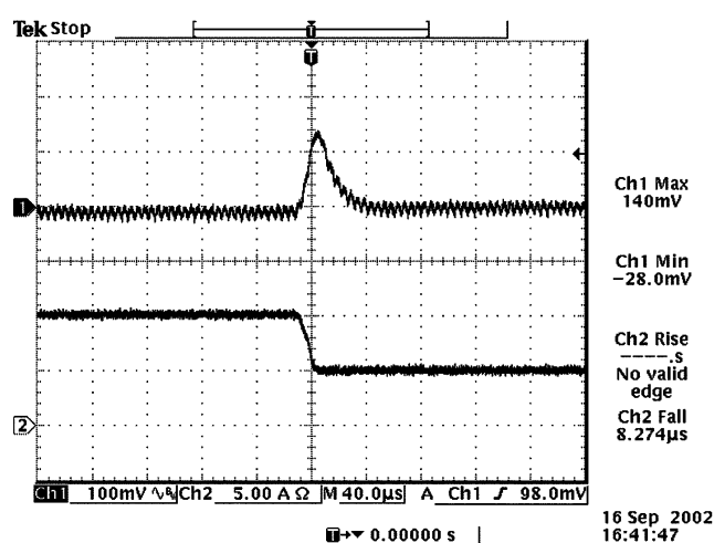
Vout=1.2V 100% to 50% load transients at 12V input and T_a=25^\circ C
