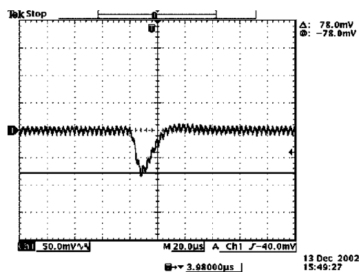
Vout=0.9V 50% to 100% load transients at 5V input and Ta=25° C
