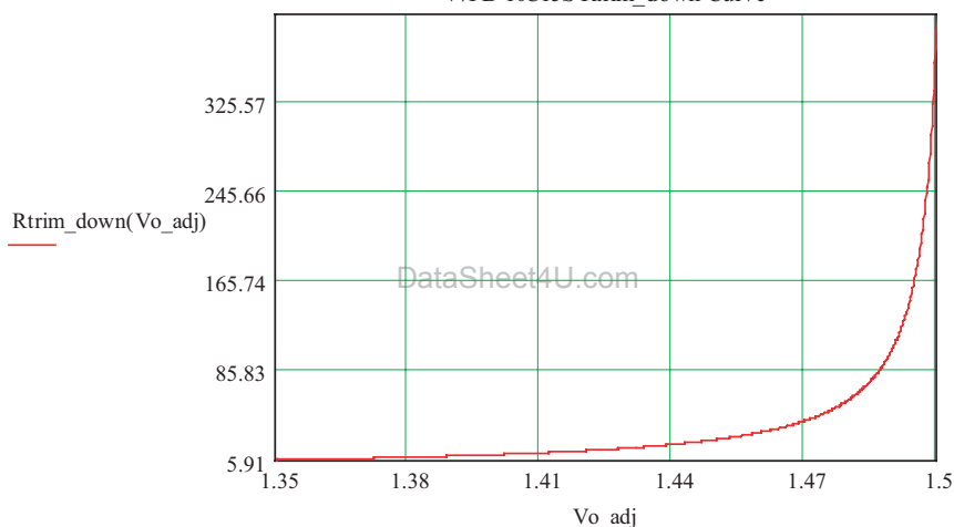
V7PB-10C15S Rtrim_down Curve
