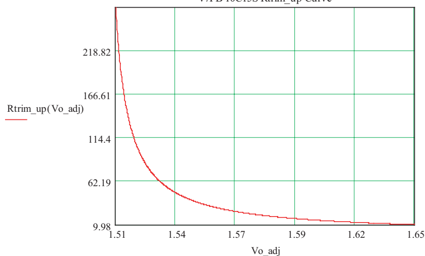
V7PB-10C15S Rtrim_up Curve
