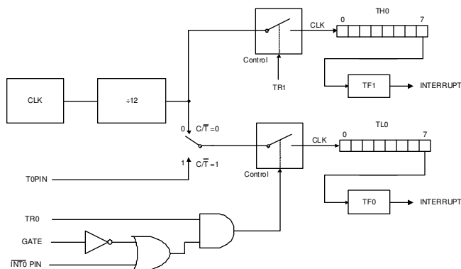
FIGURE 14: TIMER/COUNTER 0 MODE 3
