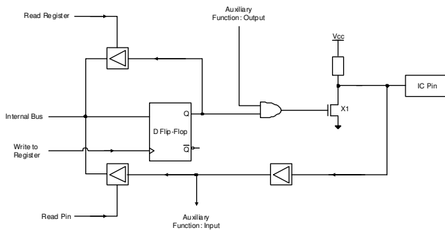
FIGURE 11: P3 PORT STRUCTURE
