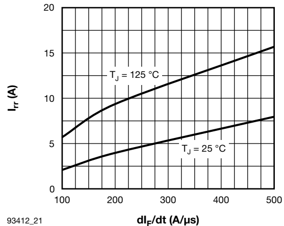
Fig. 21 - Typical I_{rr} Chopper Diode vs. dl_F/dt V_{rr} = 200\text{ V} , I_F = 60\text{ A}
