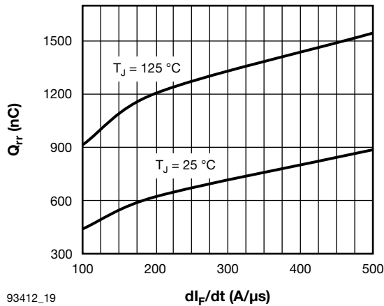
Fig. 19 - Typical Q_{rr} Antiparallel Diode vs. dl_F/dt V_{rr} = 200\text{ V} , I_F = 60\text{ A}
