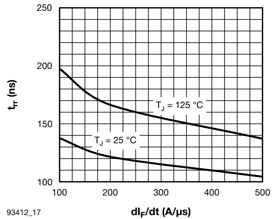
Fig. 17 - Typical t rr Antiparallel Diode vs. di F /dt V rr = 200 V, I F = 60 A
