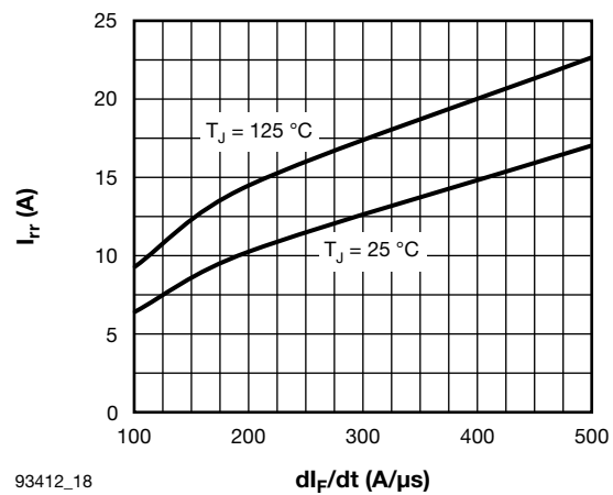
Fig. 18 - Typical I rr Antiparallel Diode vs. di F /dt V rr = 200 V, I F = 60 A
