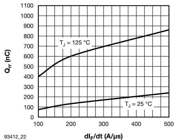
Fig. 22 - Typical Q_{rr} Chopper Diode vs. dl_F/dt V_{rr} = 200\text{ V} , I_F = 40\text{ A}
