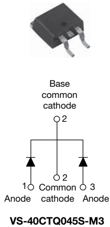
TO 263AB (D 2 PAK)
