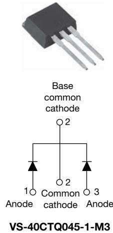
TO-262AA
