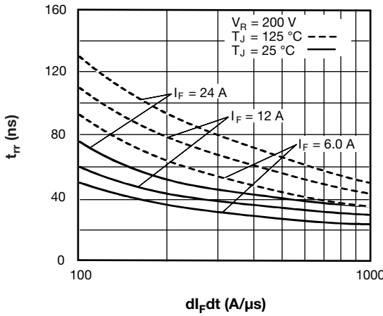
Fig. 14 - Typical Reverse Recovery Time vs. di/dt
