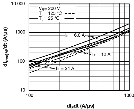
Fig. 17 - Typical dI_{(rec)M}/dt vs di/dt
