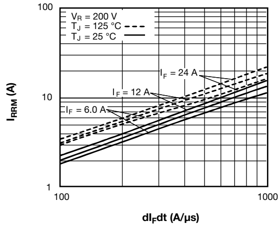
Fig. 15 - Typical Recovery Current vs. di/dt
