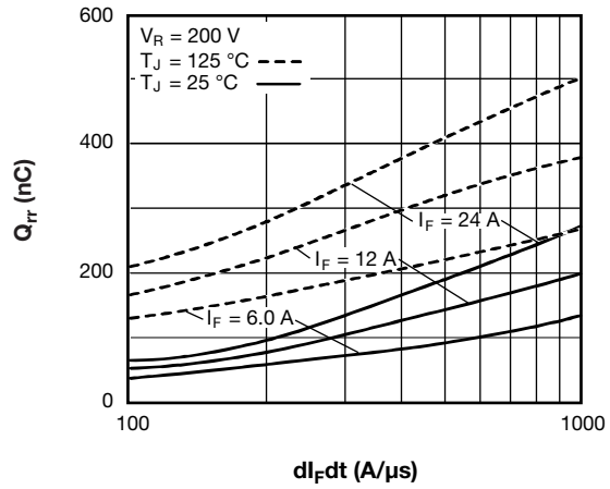
Fig. 16 - Typical Stored Charge vs. di/dt
