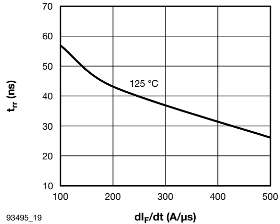
Fig. 19 - Typical PFC Diode Reverse Recovery Time vs. di/dt V R = 200 V, I F = 10 A
