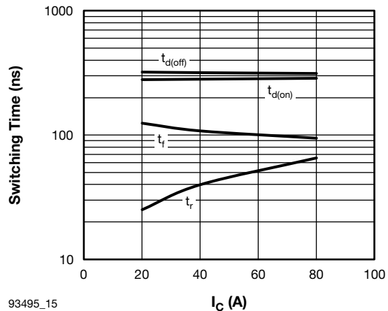
Fig. 15 - Typical PFC IGBT Switching Time vs. I_C (with Freewheeling D3 - D4 PFC Diode) T_J = 125\text{ }^\circ\text{C} , V_{CC} = 400\text{ V} , R_g = 4.7\text{ }\Omega , V_{GE} = 15\text{ V} , L = 500\text{ }\mu\text{H}
