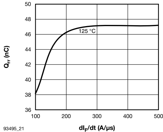
Fig. 21 - Typical PFC Diode Reverse Recovery Charge vs. di/dt V R = 200 V, I F = 10 A
