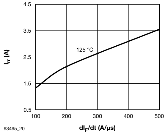
Fig. 20 - Typical PFC Diode Reverse Recovery Current vs. di/dt V R = 200 V, I F = 10 A
