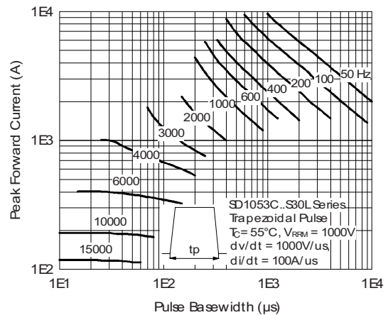
Fig. 39 - Frequency Characteristics
