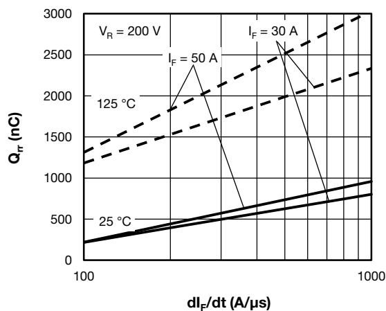
Fig. 8 - Typical Stored Charge vs. di/dt (per Leg)
