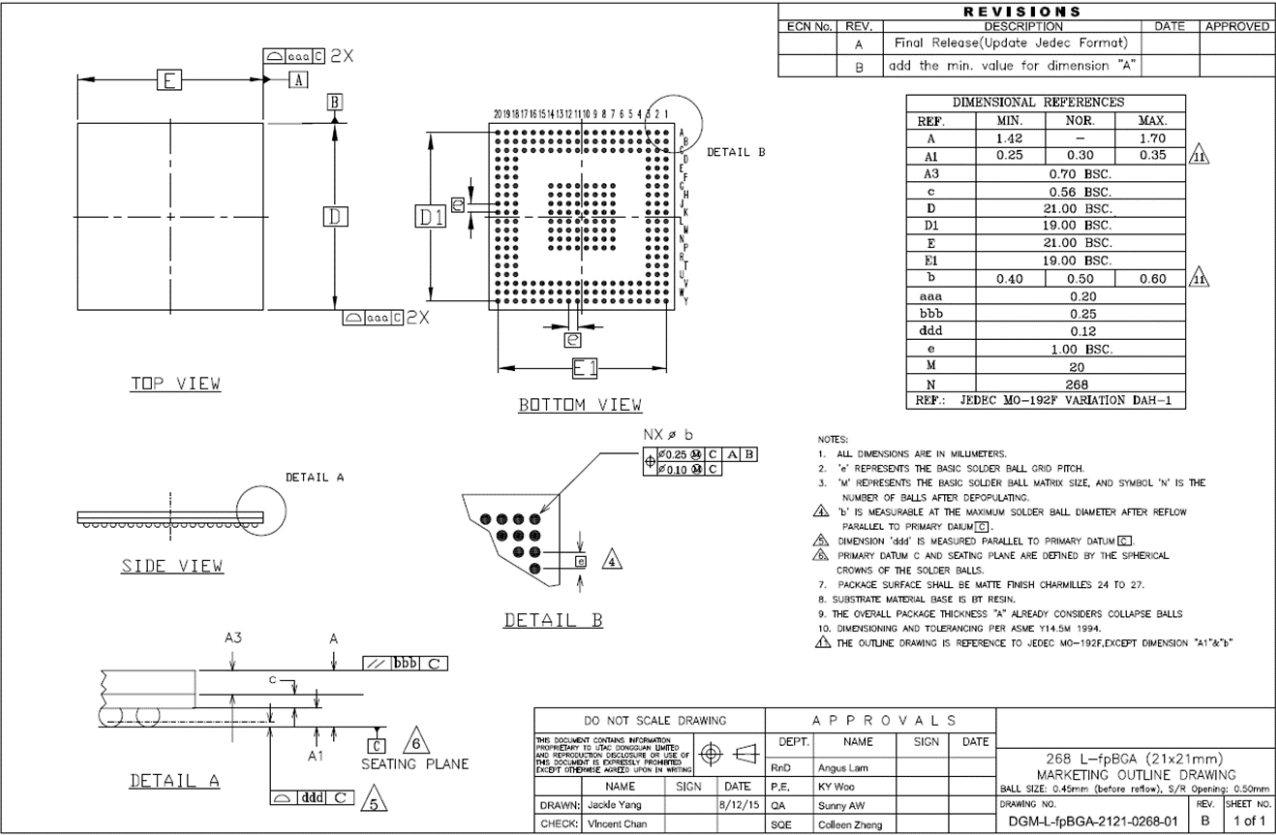
Figure 21: VS100RX – Mechanical Information
