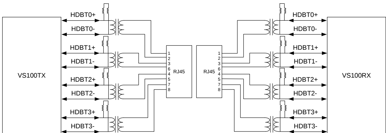
Figure 15: VS100RX and VS100TX HDBaseT Connection Example
