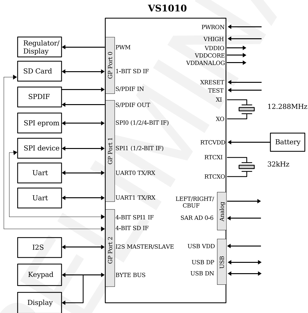
Figure 7: VS1010c external interfaces
