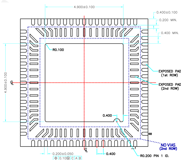
Figure 11: VS1010d bottom view, QFN-68, obsolete. Do not use this package revision as a basis for new PCB design
