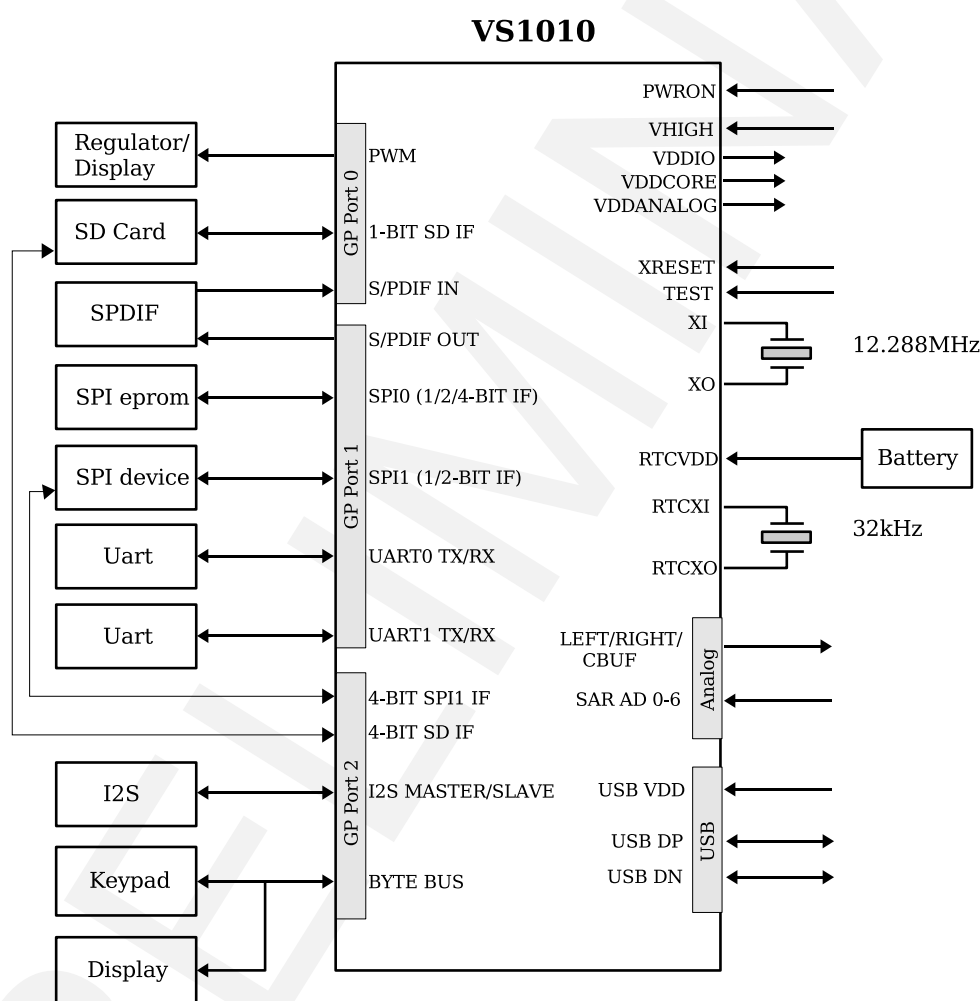
Figure 14: VS1010d external interfaces
