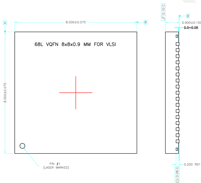
Figure 10: VS1010d top and side views, QFN-68, obsolete. Do not use this package revision as a basis for new PCB design
