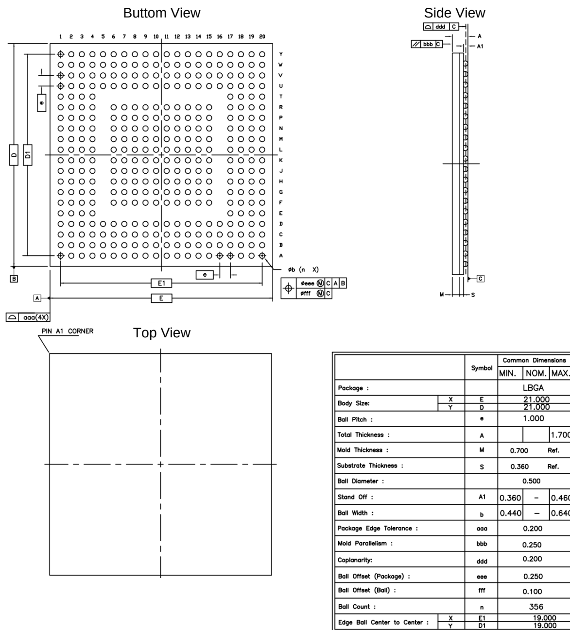
Figure 15: VS2010TX Mechanical Information (all dimensions in mm)
