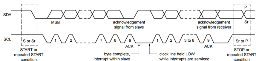
Figure 21: Native I 2 C Data Transfer (Ref: I2C-Bus Specification, Rev.6)
