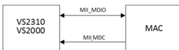
Figure 16: MDIO Topology
