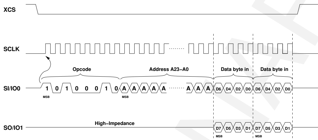
Figure 24: SPI Dual-Input Write
