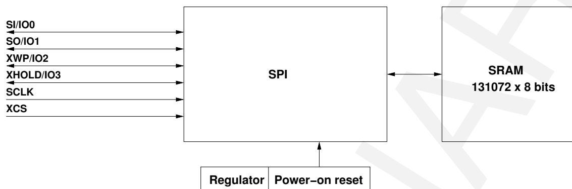
Figure 10: Device Organization
