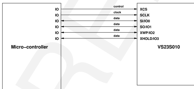
SPI Dual-I/O connection
