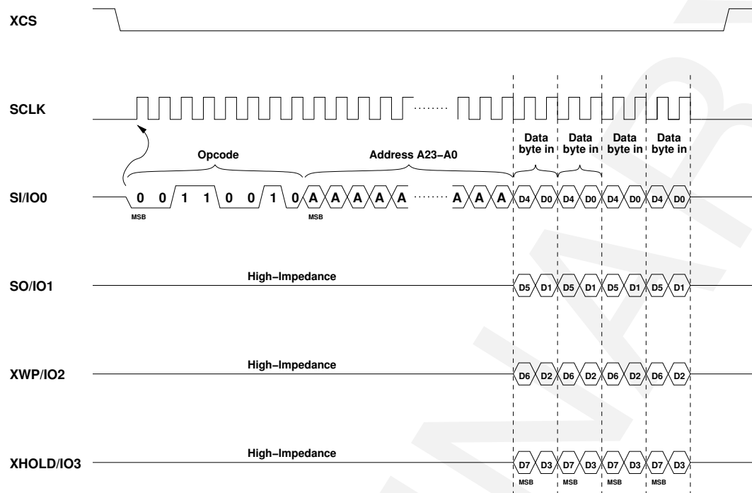
Figure 26: SPI Quad-Input Write
