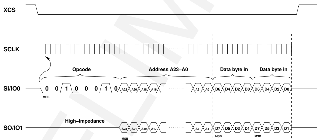
Figure 25: SPI Dual-Input, Dual Address Write
