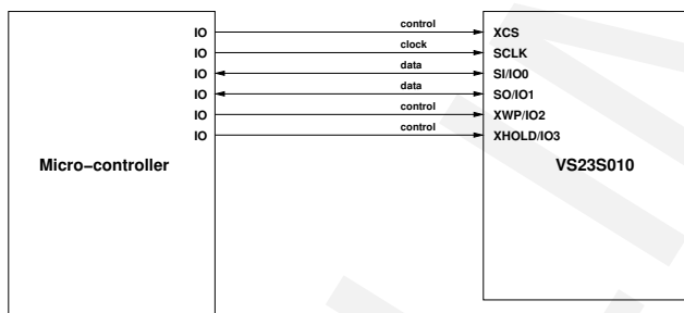
SPI connection, basic configuration
