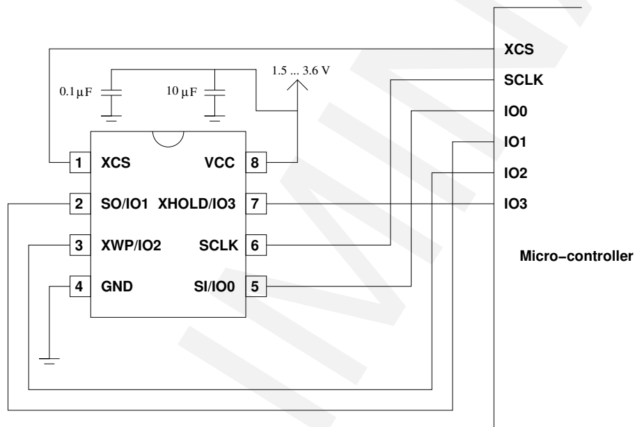
Figure 9: Connection example
