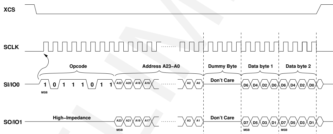
Figure 20: SPI Dual-Output Read, Dual Address
