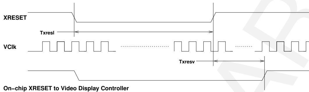
Figure 8: XRESET Timing
