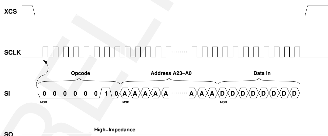
Figure 33: SPI Write
