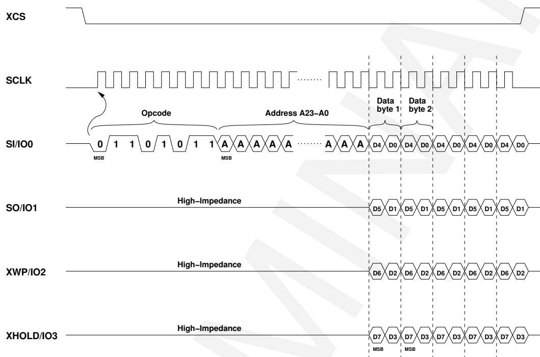
Figure 31: SPI Quad-Output Read
