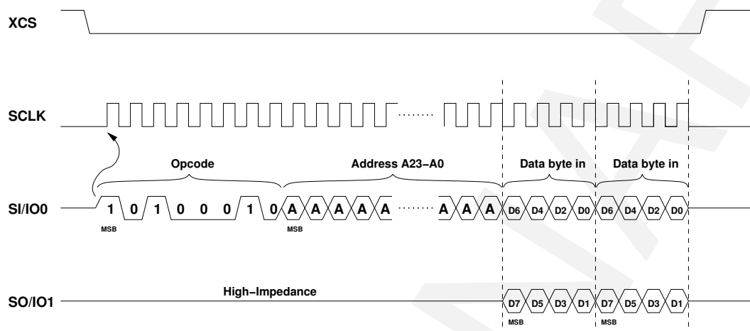
Figure 34: SPI Dual-Input Write
