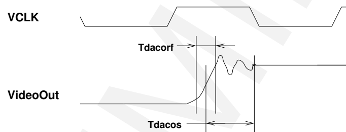
Figure 9: VideoOut Timing
