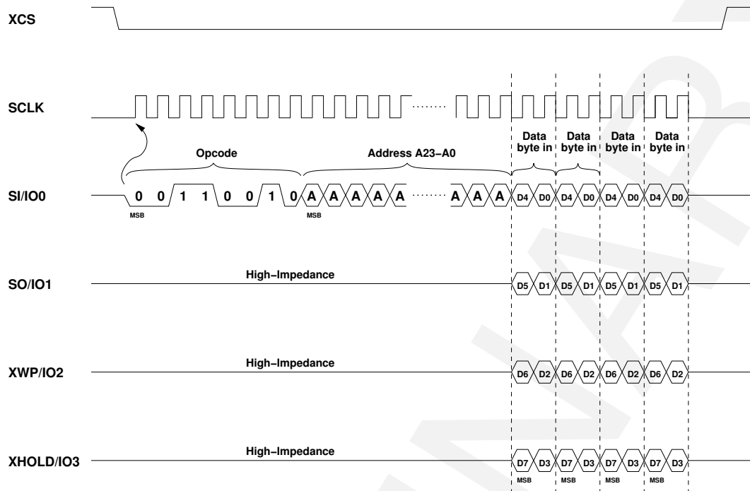
Figure 30: SPI Quad-Input Write
