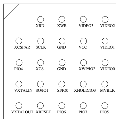
Figure 1: pin out (top view, not to scale)
