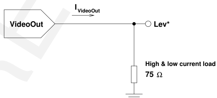
Figure 10: VideoOut Level Measurement
