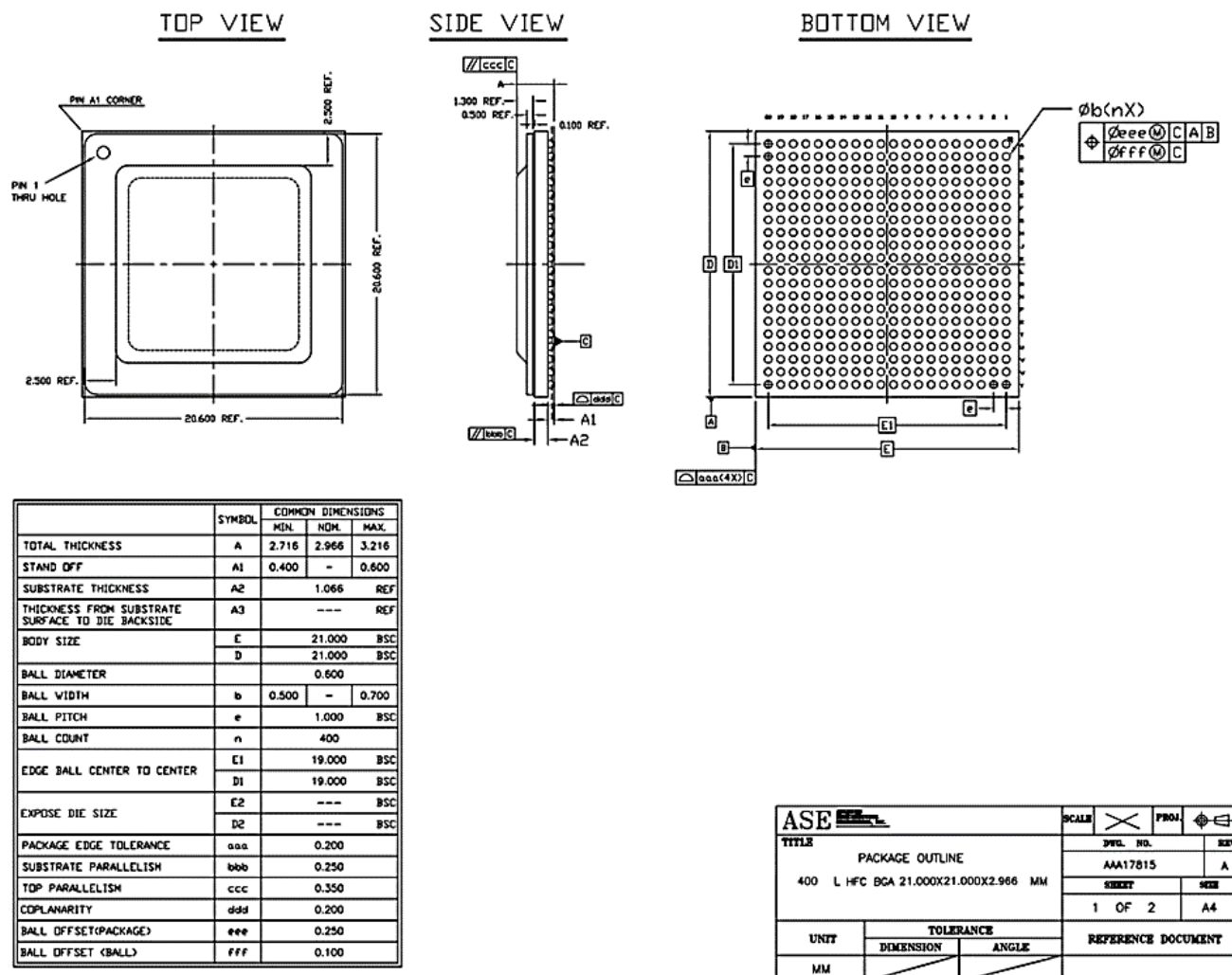
Figure 29: VS300R Mechanical Information (all dimensions in mm)
