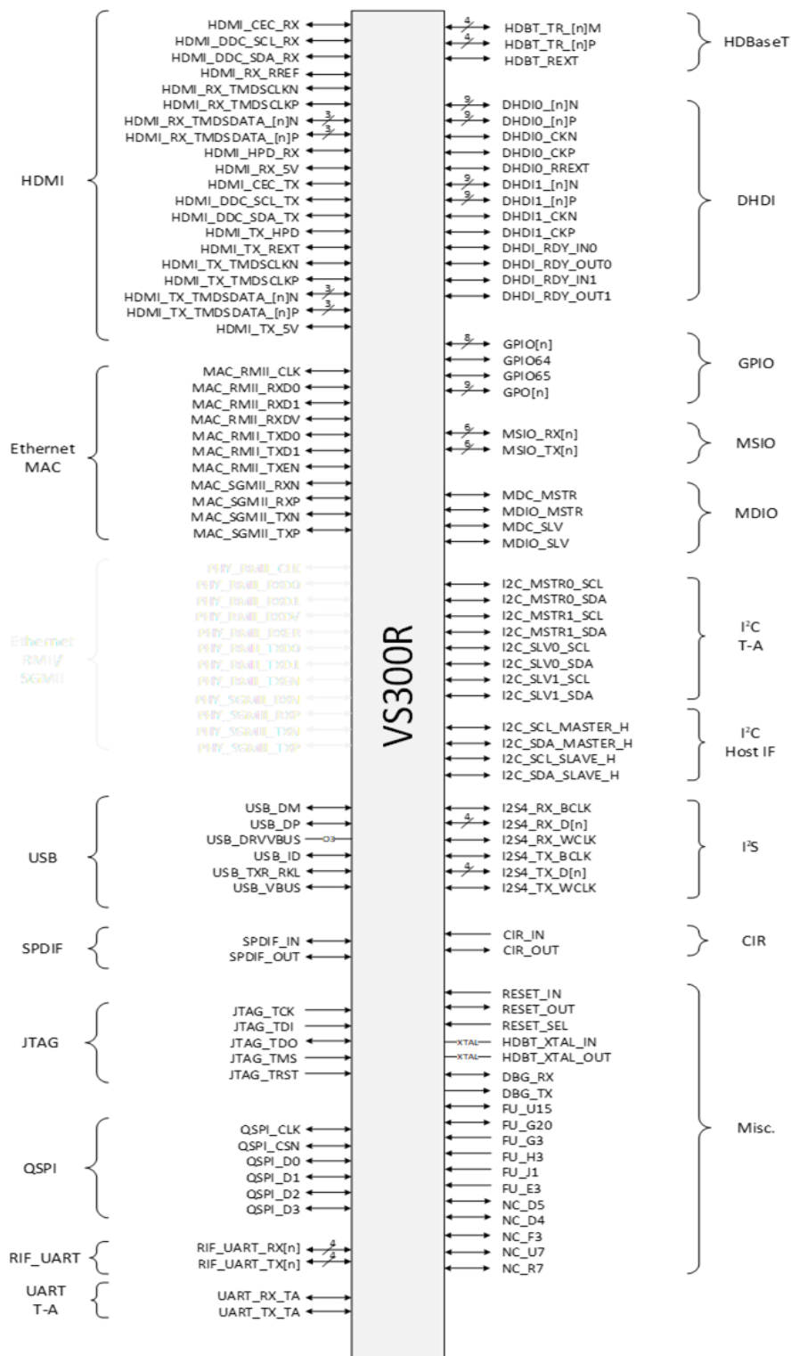
Figure 8: VS300R I/F Signal Block Diagram
