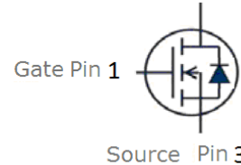
Drain Pin 2
