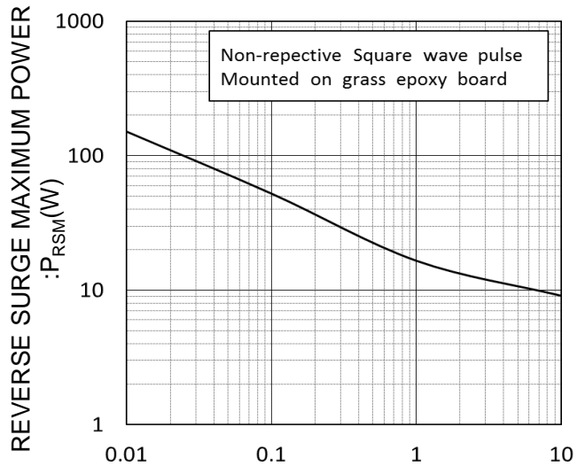
P_{RSM} - t CHARACTERISTICS
