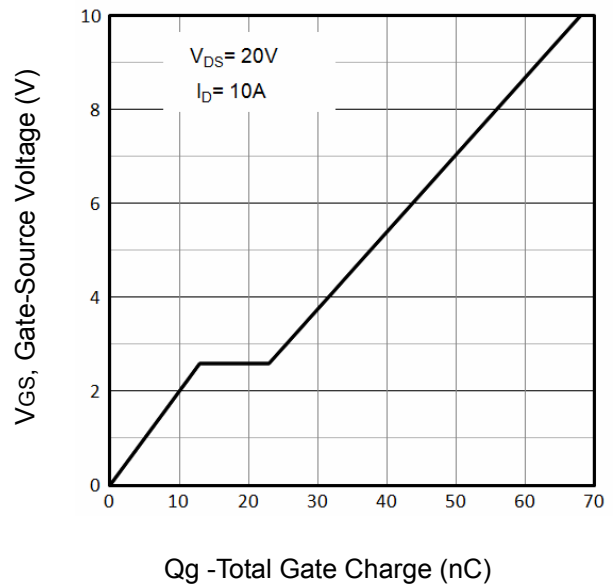
Fig8. Typical Gate Charge Vs. Gate-Source
