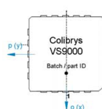
VS9000 top view
