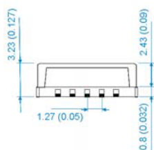
VS9000 side view
