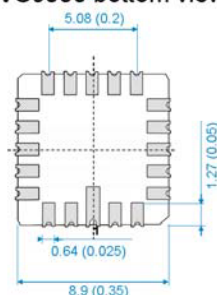
VS9000 bottom view
