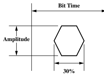
Receiver Input Eye Diagram Jitter Mask
