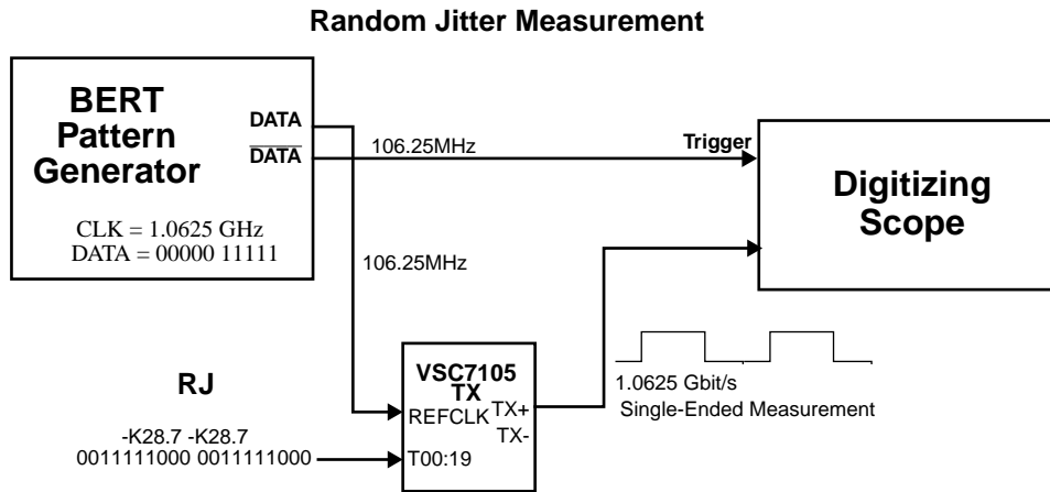
Figure 13: Transmitter Jitter Measurement Method
